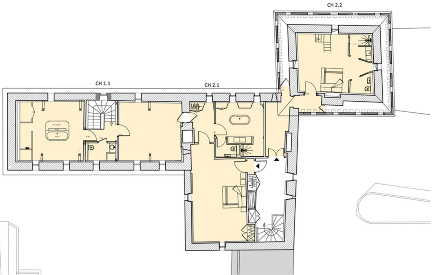
Plan combles - GRAND LOGIS
